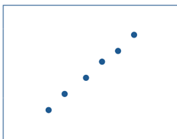
Image Space
