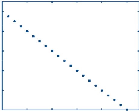
Image Space
